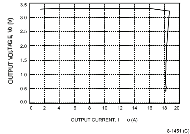
Figure 6. Typical JW075F Output Characteristics at Room Temperature
