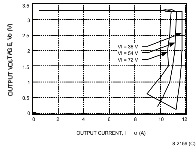
Figure 5. Typical JW050F Output Characteristics at Room Temperature
