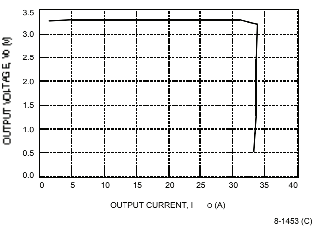
Figure 8. Typical JW150F Output Characteristics at Room Temperature
