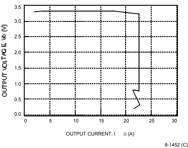
Figure 7. Typical JW100F Output Characteristics at Room Temperature
