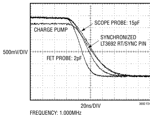
Figure 24. CLKOUT Fall Time
