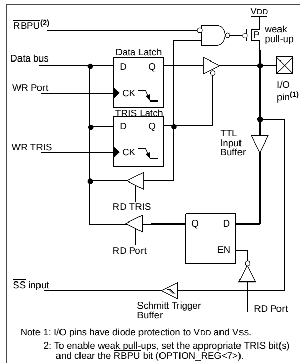
FIGURE 3-5: BLOCK DIAGRAM OF RB1/ \overline{\text{SS}} PIN
