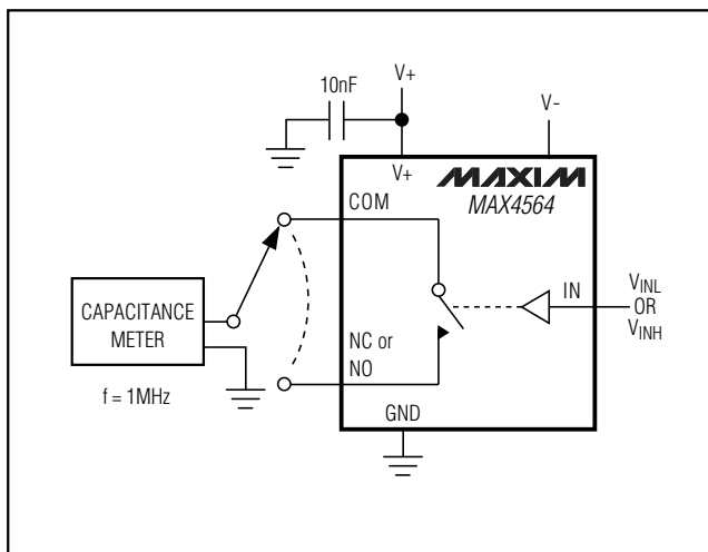
Figure 6. Channel Off/On-Capacitance
