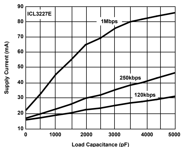
Figure 7. Supply Current vs Load Capacitance When Transmitting Data
