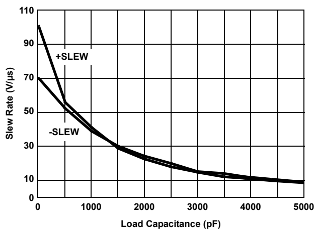
Figure 5. Slew Rate vs Load Capacitance
