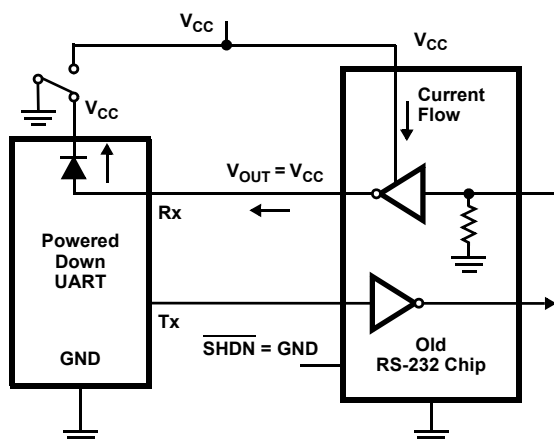
Figure 11. Power Drain Through Powered Down Peripheral
