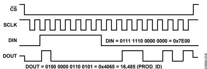
Figure 16. SPI Read Example, Second 16-Bit Sequence
