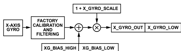
Figure 22. User Calibration Signal Path, Gyroscopes
