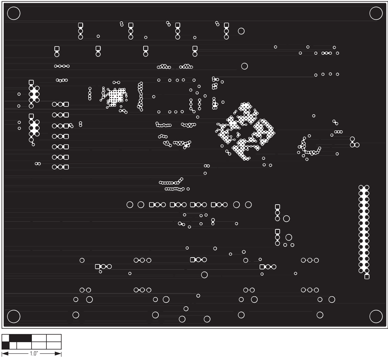
Figure 15. MAX11103 EV Kit PCB Layout—Layer 8
