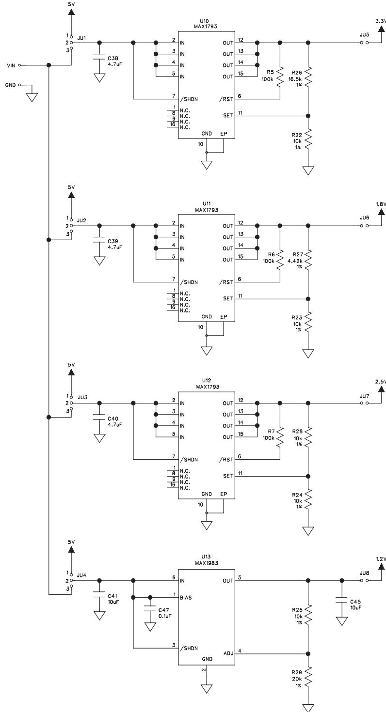
Figure 6k. MAX11103 EV Kit Schematic (Sheet 11 of 12)
