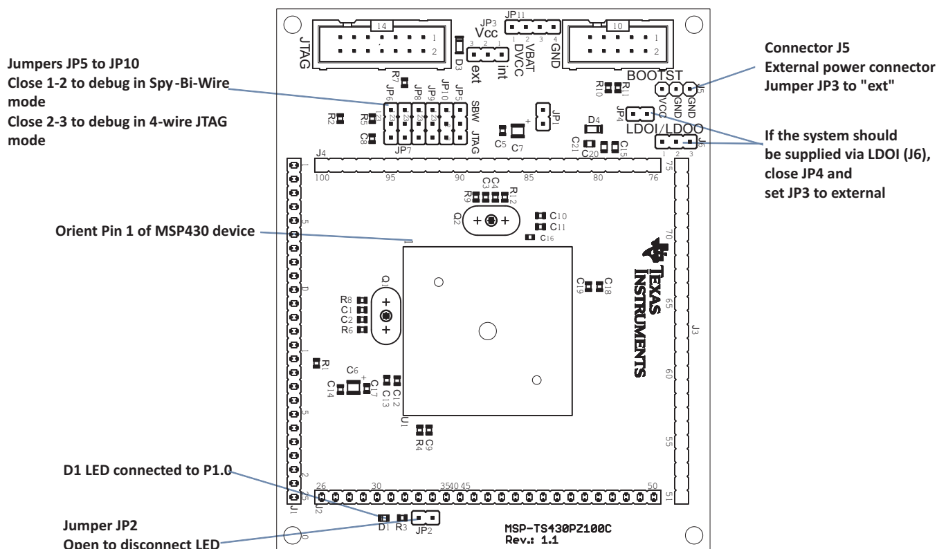
Figure B-54. MSP-TS430PZ100C Target Socket Module, PCB
