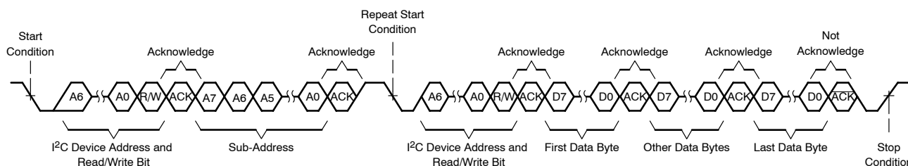
Figure 4–5. Multiple Byte Read Transfer
