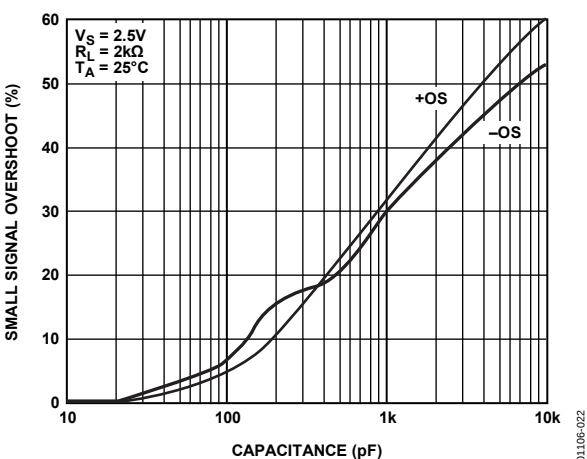
Figure 21. Small Signal Overshoot vs. Load Capacitance
