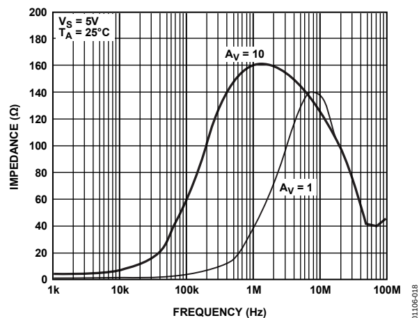
Figure 17. Closed-Loop Output Impedance vs. Frequency
