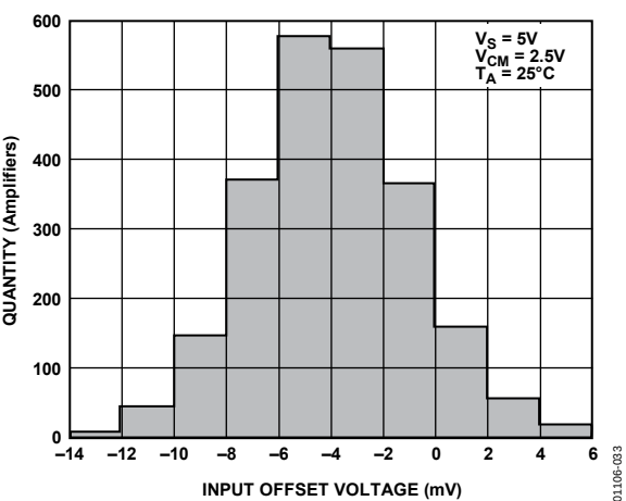
Figure 32. Input Offset Voltage Distribution
