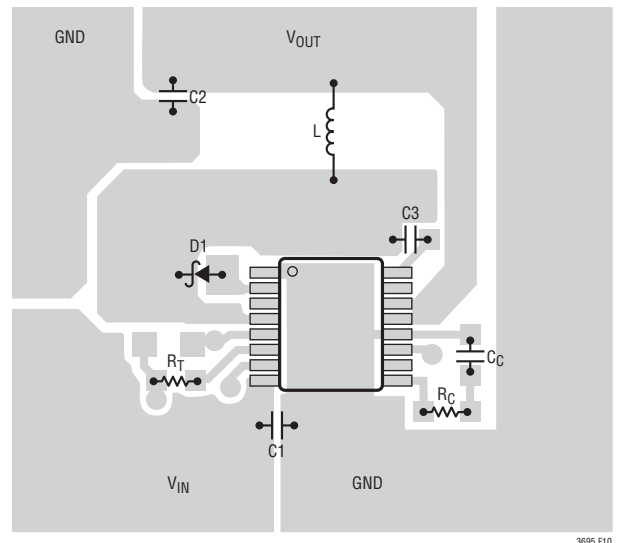
Figure 10. A Good PCB Layout Ensures Proper, Low EMI Operation (LT3695-3.3, LT3695-5)
