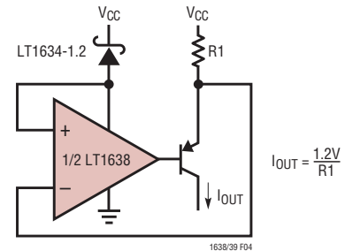
Figure 4. Current Source
