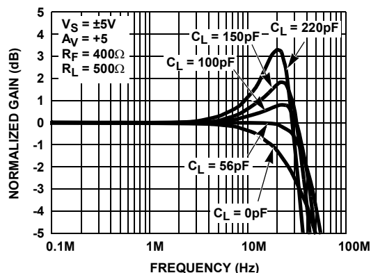
FIGURE 13. GAIN vs FREQUENCY FOR VARIOUS C_{LOAD} ( A_V = +5 )
