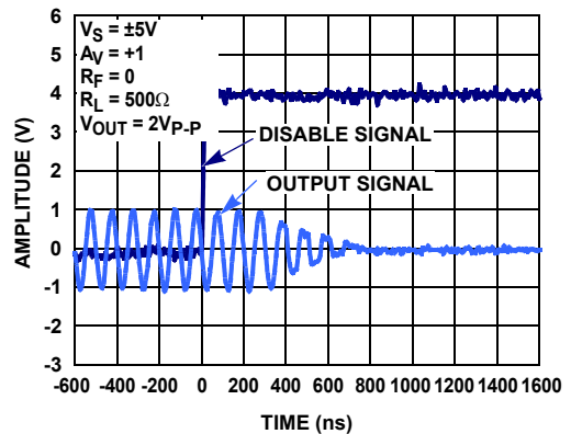
FIGURE 30. TURN-OFF TIME
