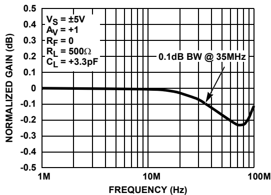
FIGURE 3. 0.1dB BANDWIDTH
