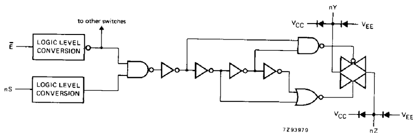
Fig. 5 Schematic diagram (one switch).
