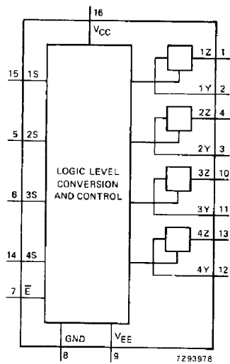
Fig. 4 Functional diagram.
