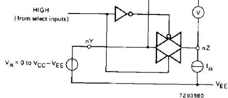
Fig. 8 Test circuit for measuring R_{ON} .
