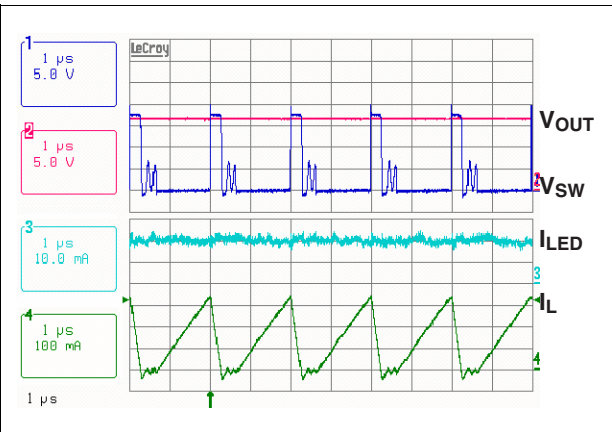
Figure 15. Typical waveform
