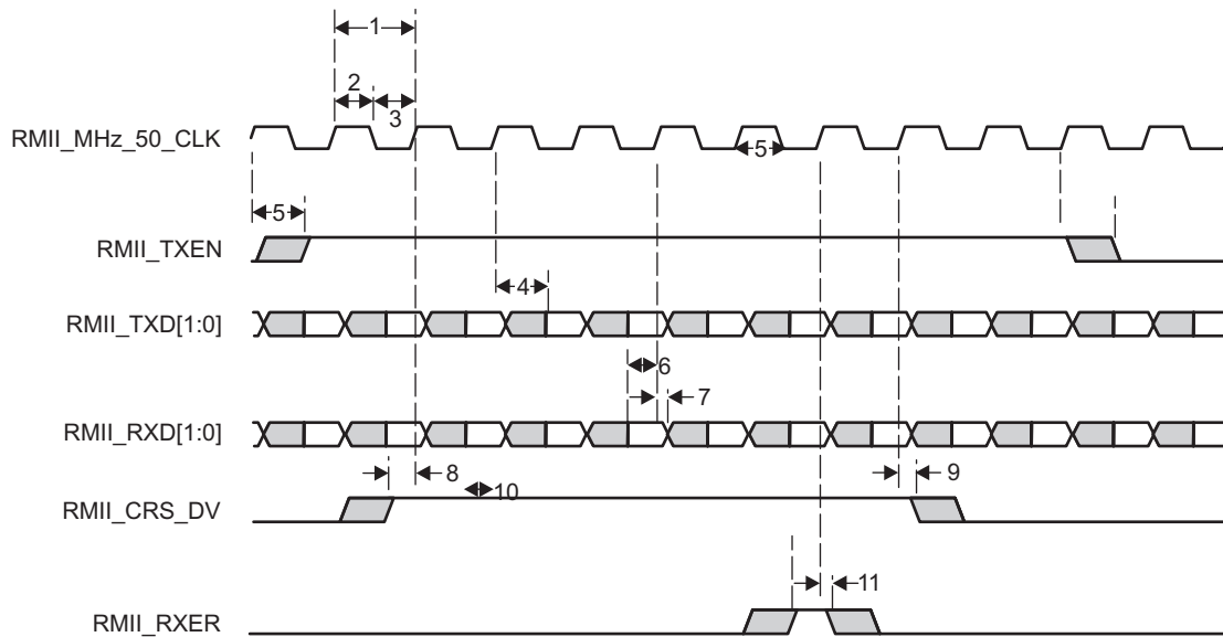
Figure 5-24. RMII Timing Diagram
