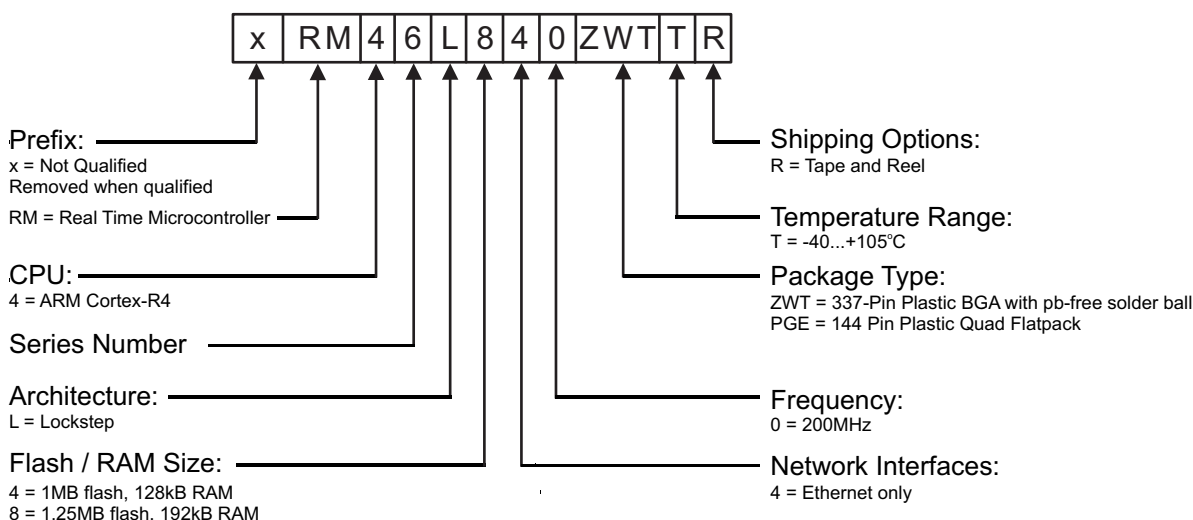
Figure 6-1. RM46Lx40 Device Numbering Conventions
