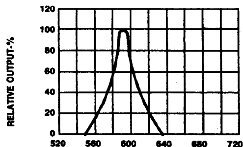
Fig.2 SPECTRAL RESPONSE
