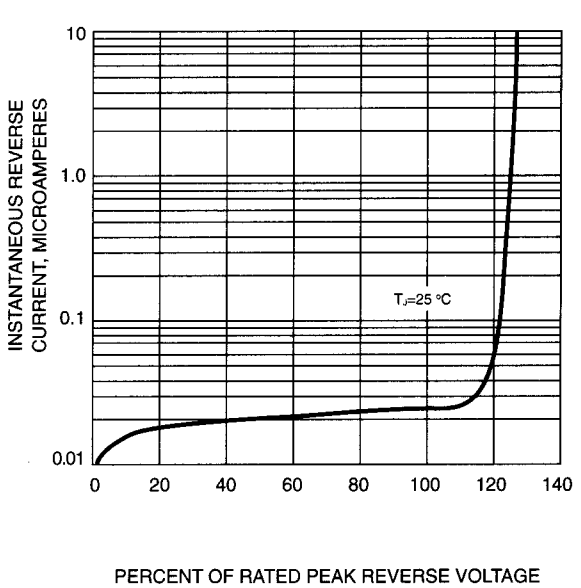
FIG. 4-TYPICAL REVERSE CHARACTERISTICS
