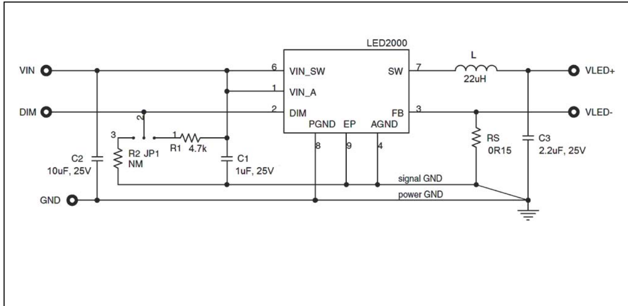
Figure 1. STEVAL-ILL051V1 circuit schematic
