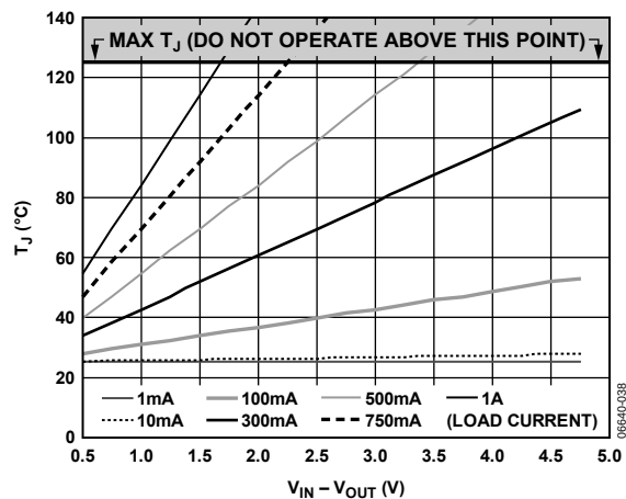
Figure 39. 500 mm² of PCB Copper, T_A = 25^\circ\text{C} , LFCSP
