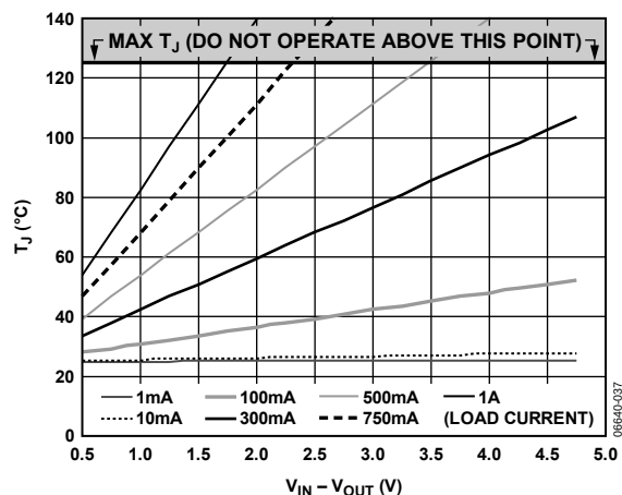
Figure 38. 0 mm² of PCB Copper, T_A = 25^\circ\text{C} , SOIC
