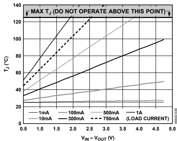
Figure 37. 100 mm² of PCB Copper, T_A = 25^\circ\text{C} , SOIC
