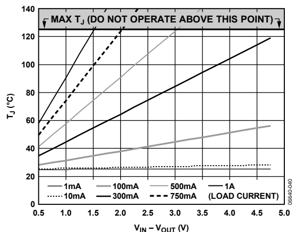
Figure 41. 0 mm² of PCB Copper, T_A = 25^\circ\text{C} , LFCSP
