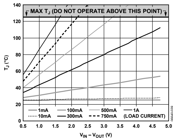
Figure 40. 100 mm² of PCB Copper, T_A = 25^\circ\text{C} , LFCSP
