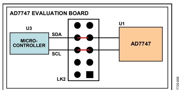
Figure 2. Evaluation Board in the Default Configuration
