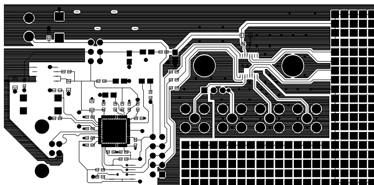
Eval-AD7747EBZ Rev. 0 (Component Side View) Component Side
