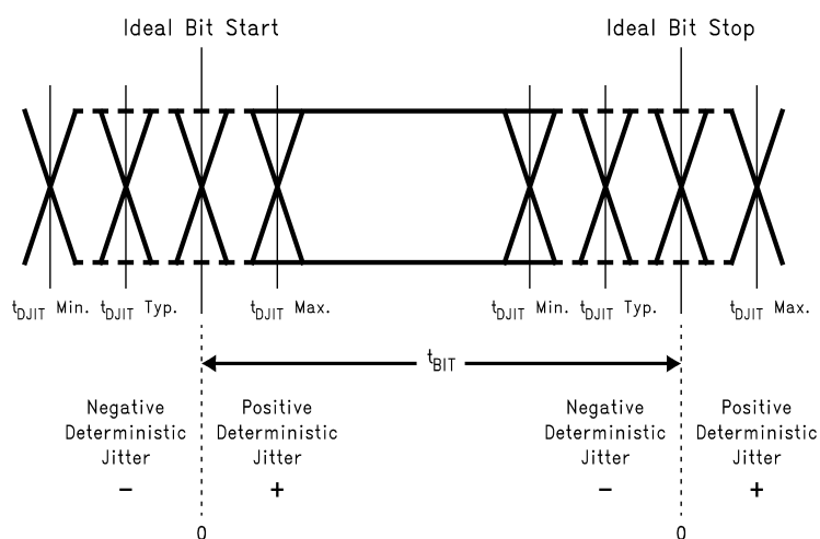
Figure 10. Deterministic Jitter and Ideal Bit Position
