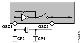
Figure 32. Oscillator Circuit on the ADF7021-N
