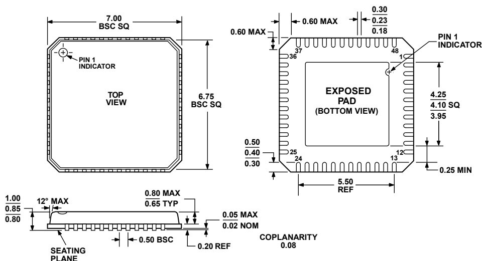
Figure 79. 48-Lead Lead Frame Chip Scale Package [LFCSP_VQ]
