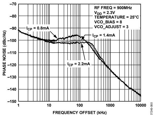
Figure 11. Phase Noise Response at 900 MHz, V_{DD} = 2.3 V
