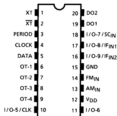
TC9257P, TC9257F
