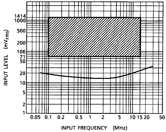
IF IN Frequency Characteristics
