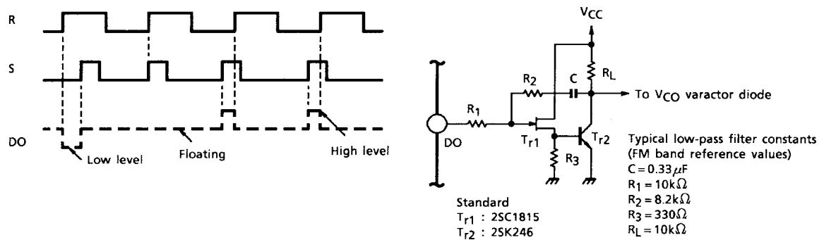
Figure 8 DO Output Timing Chart
