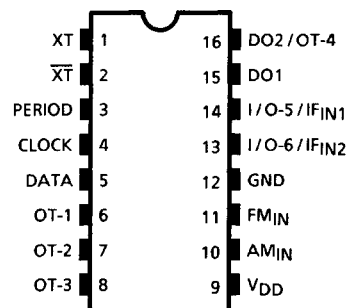
TC9256P, TC9256F
