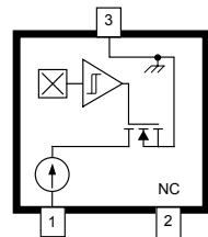
LH Package [1]
