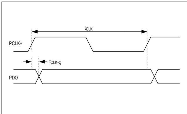
Figure 3. Timing Parameters
