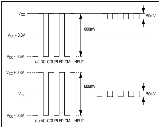
Figure 1. Input Amplitude
