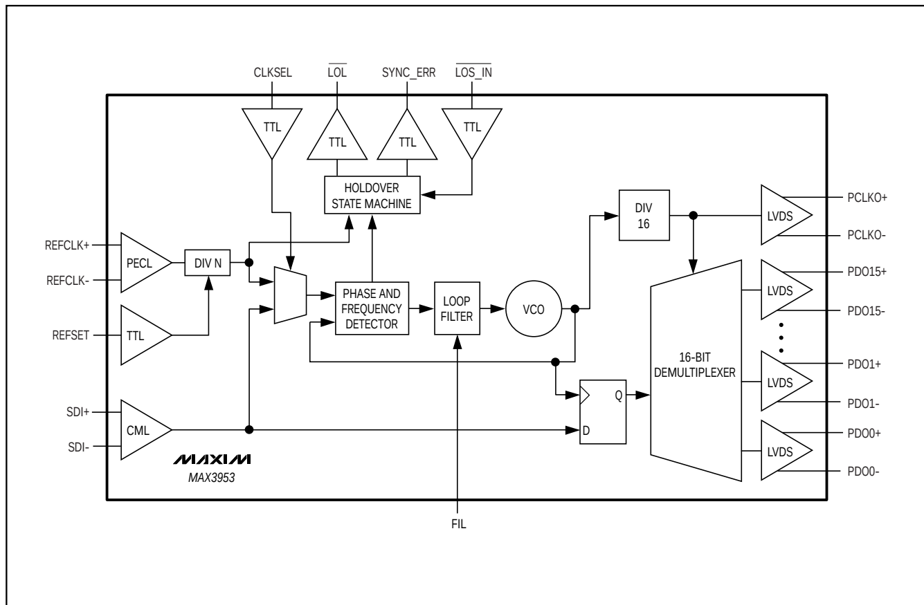
Functional Diagram
