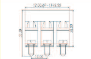
Dimensions - mm
