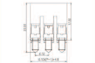
Dimensions - mm
