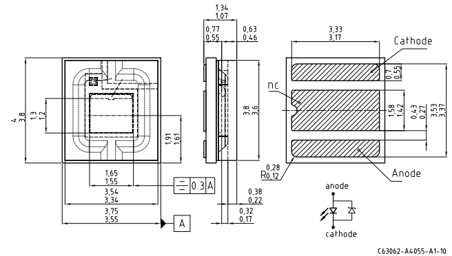
Figure 4: OSLO Black Flat
