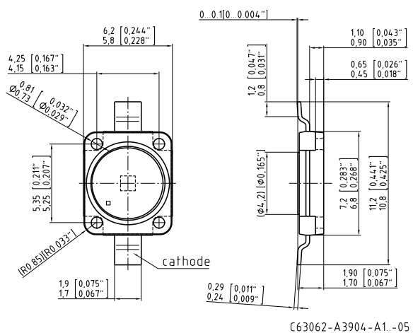
Figure 6: Golden DRAGON
