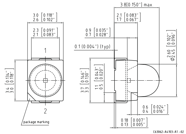
Figure 42: MULTILED
