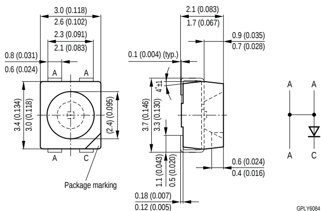
Figure 11: Power TOPLED
