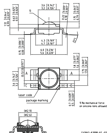
Figure 59: Advanced Power TOPLED Plus
