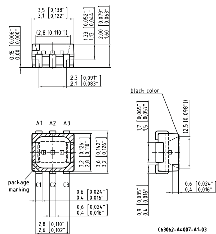
Figure 42: MULTILED
