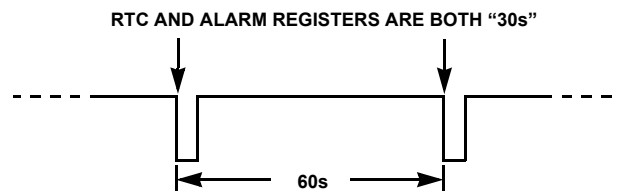
FIGURE 14. \overline{\text{IRQ}}/\text{FOUT} WAVEFORM
