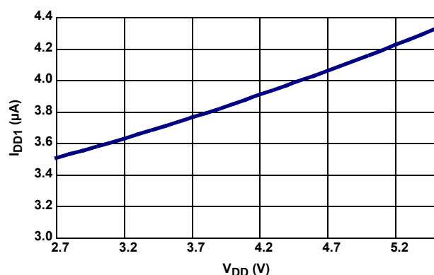
FIGURE 6. I_{DD1} vs V_{DD}
