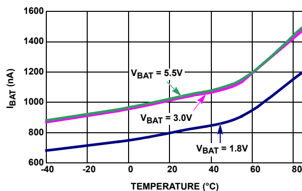
FIGURE 4. I_{BAT} vs TEMPERATURE
