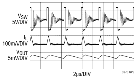
Switching Waveforms, Burst Mode Operation
