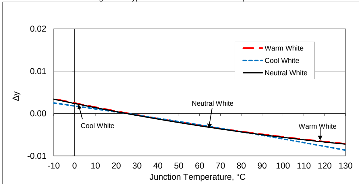
Figure 4: Typical ccx Shift vs. Junction Temperature
