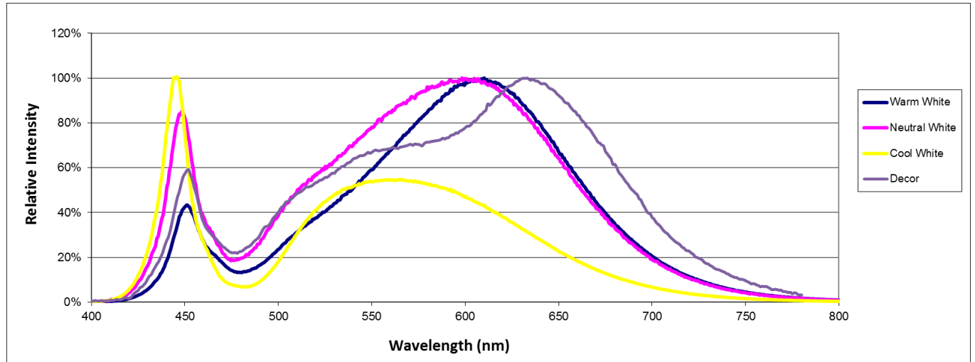
Figure 8: Typical Color Spectrum
