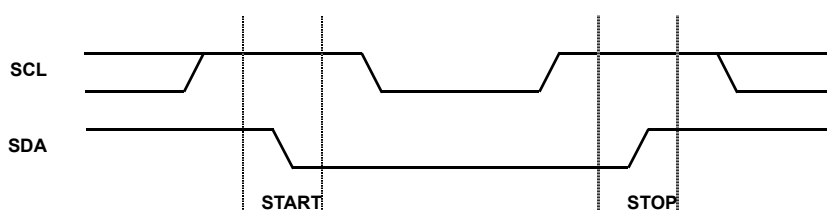
FIGURE 17. VALID START AND STOP CONDITIONS
