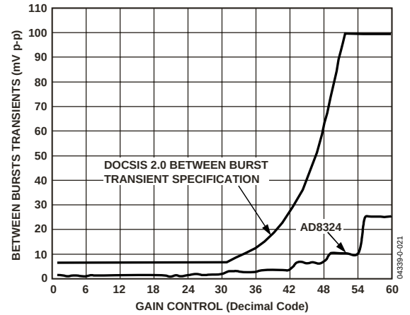
Figure 21. Between Burst Transient vs. Gain Control
