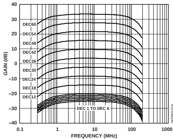
Figure 14. AC Response
