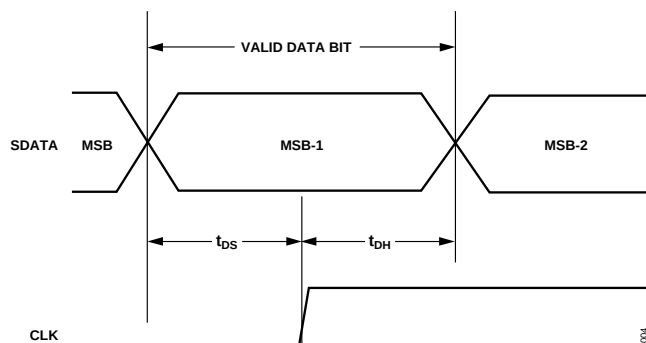
Figure 4. SDATA Timing
