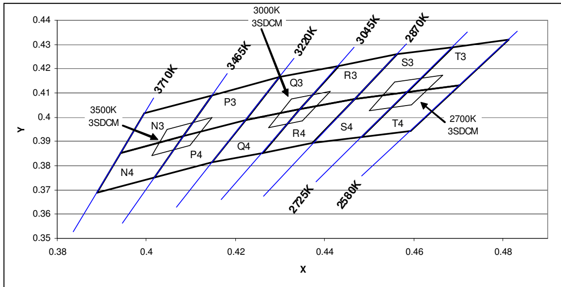
Figure 12: Graph of Warm White Test Bins in xy Color Space
