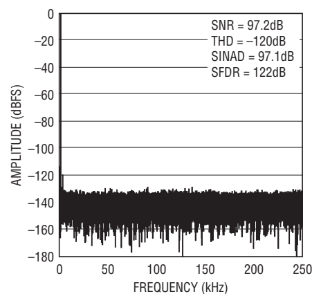
32k Point FFT f_{\text{S}} = 500\text{ksps} , f_{\text{IN}} = 2\text{kHz}
