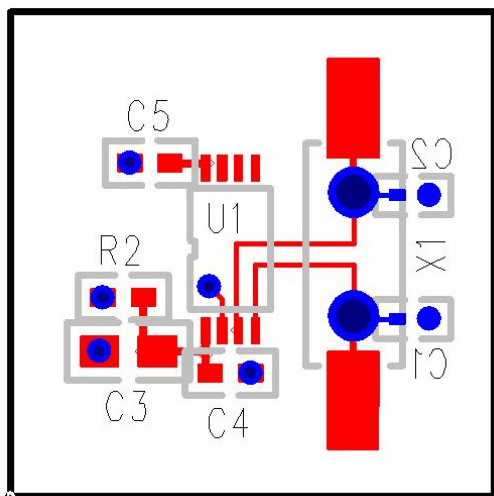
Figure 5B. ICS843SDN PC Board Layout Example
