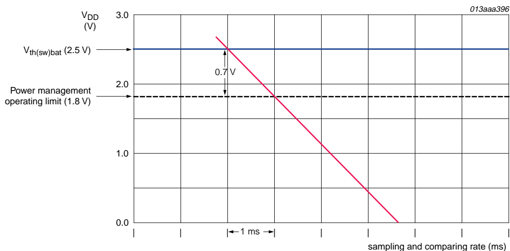
Fig 3. Supply voltage with respect to sampling and comparing rate
