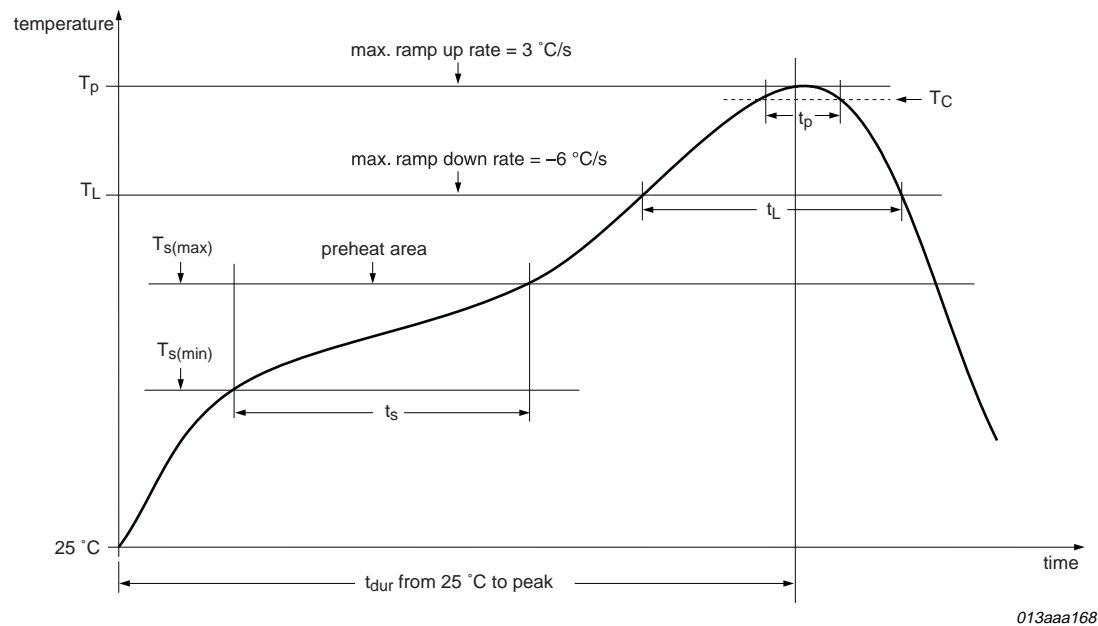
Figure not drawn to scale. The appropriate values for this graph are shown in Table 3 . Remark: The reflow profile in this document is for classification/preconditioning and not meant to specify board assembly profiles. Actual board assembly profiles should be developed based on specific process needs and board designs, but must not exceed the parameters shown in Table 3 .
