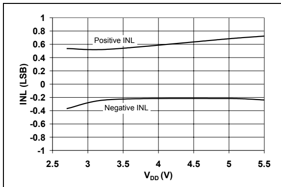
FIGURE 2-2: INL vs. V_{DD} - I^2C^{\text{TM}} Standard Mode ( f_{SCL} = 100\text{ kHz} ).
