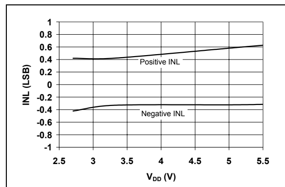
FIGURE 2-5: INL vs. V_{DD} - I^2C^{\text{TM}} Fast Mode ( f_{SCL} = 400\text{ kHz} ).
