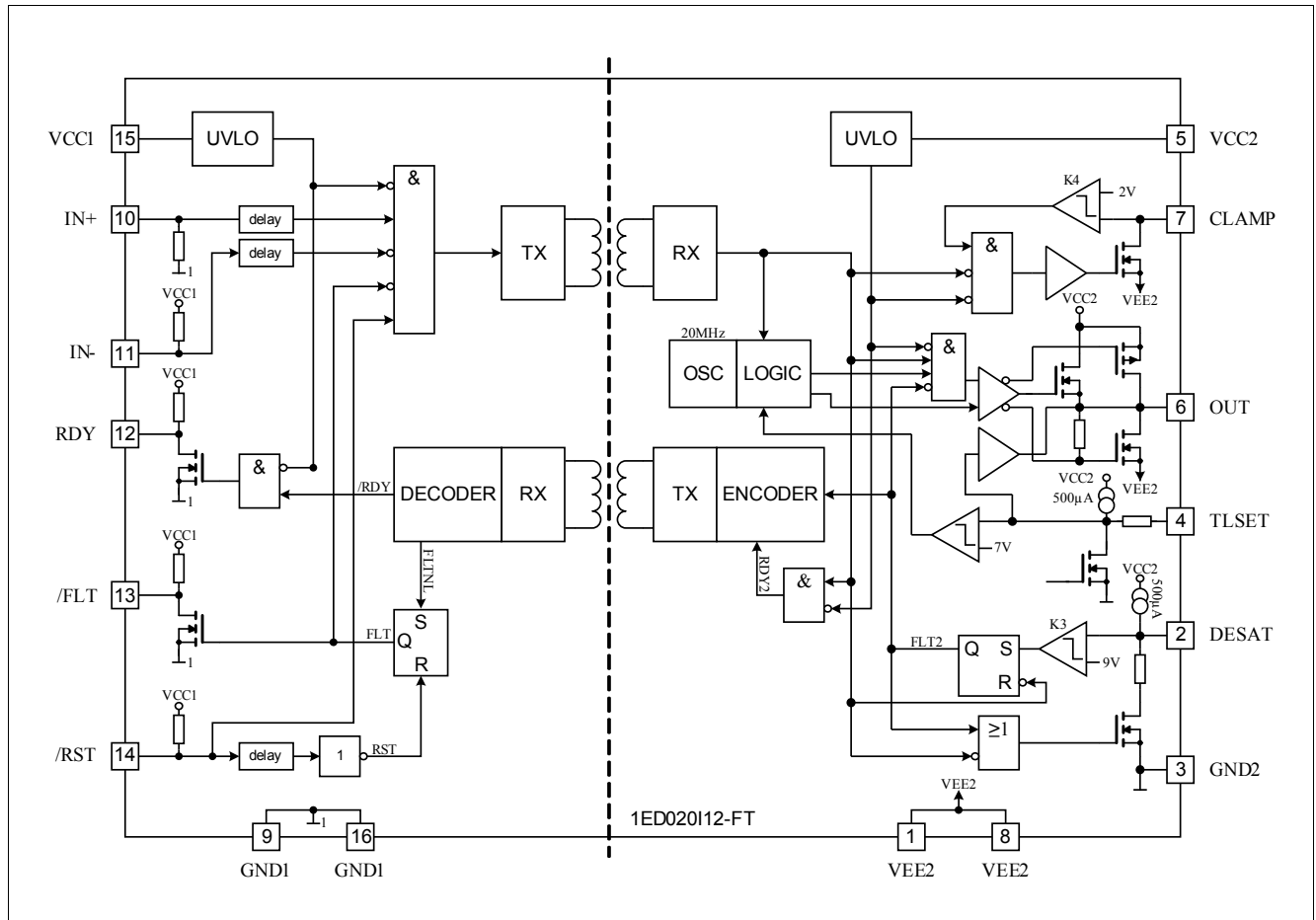
Figure 2 Block Diagram 1ED020I12-FT
