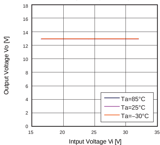
Line Regulation ( I_o=500\text{mA} )
