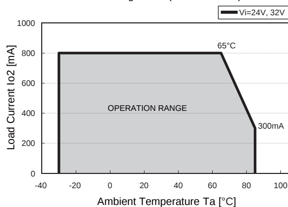
Derating Curve (With heat sink)
