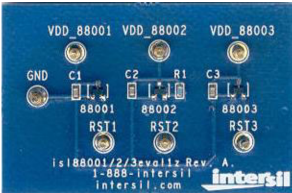
FIGURE 14. ISL88001/2/3EVAL1Z PHOTOGRAPH
