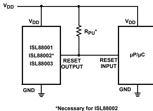
FIGURE 1. TYPICAL APPLICATION DIAGRAM
