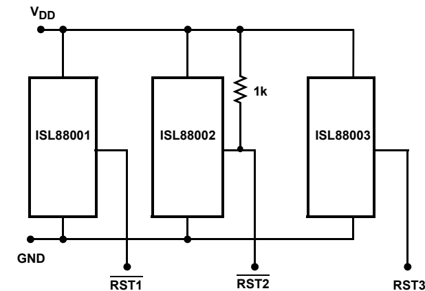
FIGURE 13. ISL88001/2/3EVAL1Z SCHEMATIC
