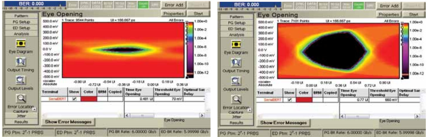
Eye Diagrams 6.0Gbps (input left, output right)
