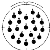
22-21 21 NO.16 CONTACTS
