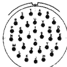
22-41 27 NO.20 14 NO.16 CONTACTS
