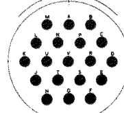
24-19 19 NO.12 CONTACTS
