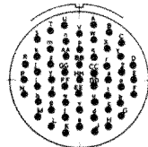
22-55 55 NO.20 CONTACTS
