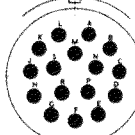
20-16 16 NO.16 CONTACTS
