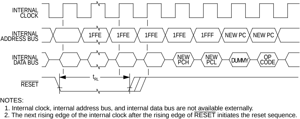
Figure 3. External Reset Timing
