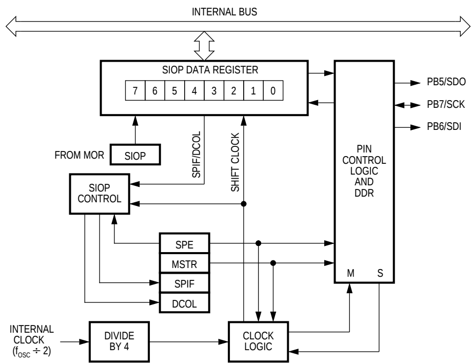
Figure 1. SIOP Block Diagram
