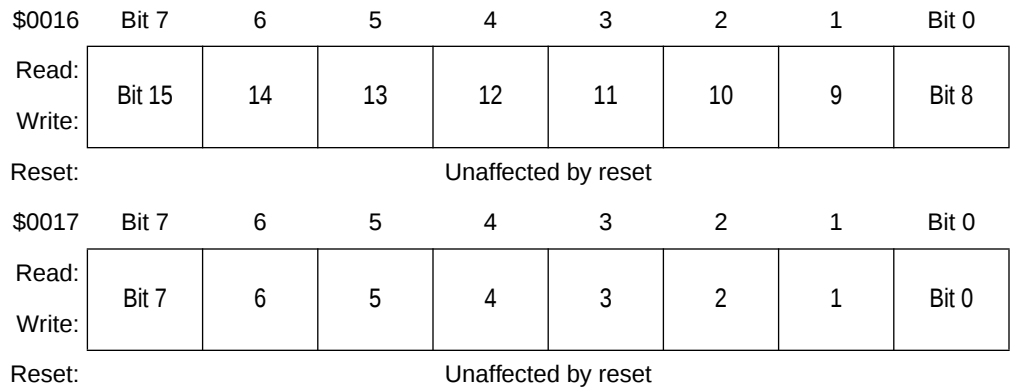
Figure 17. Output Compare Registers (OCRH and OCRL)
