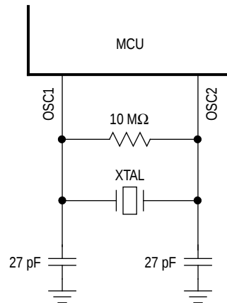
Figure 3. Crystal Connections
