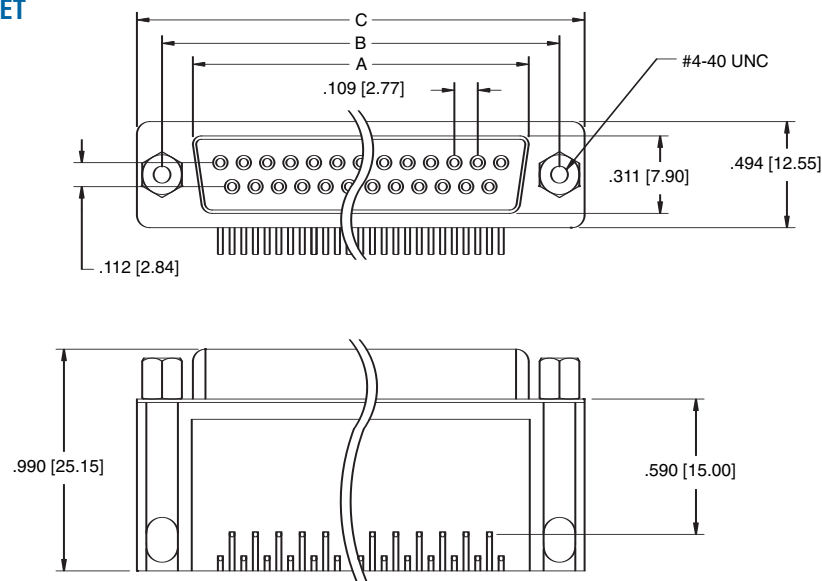
Half Flange PCB Layout for PCB mounting options (SA, SC, F)
