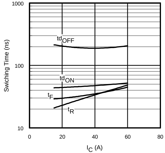
Fig. 14 - Typ. Switching Time vs. I_C T_J = 150^\circ\text{C} ; L = 200\mu\text{H} ; V_{CE} = 400\text{V} R_G = 10\Omega ; V_{GE} = 15\text{V}
