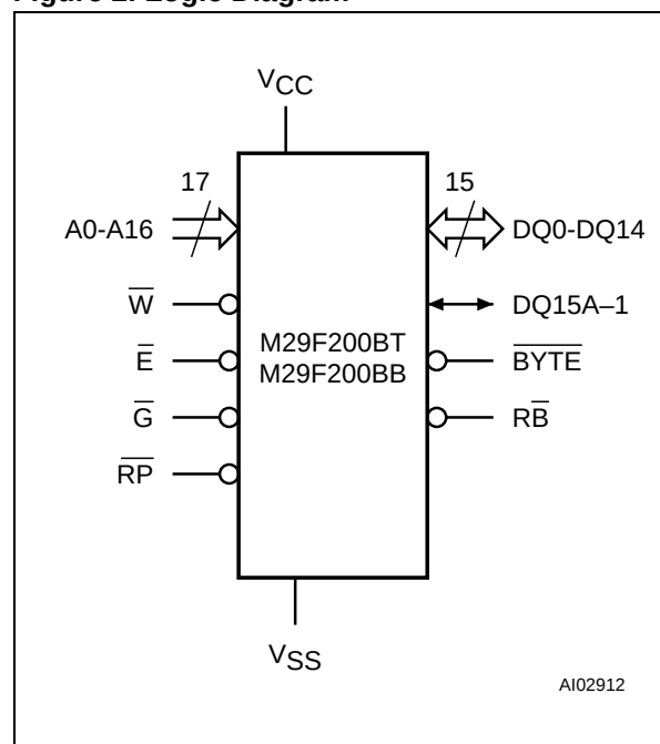
Figure 2. Logic Diagram
