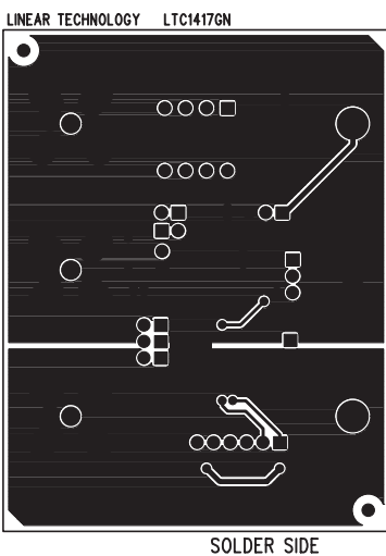
Figure 13d. Suggested Evaluation Circuit Board—Solder Side
