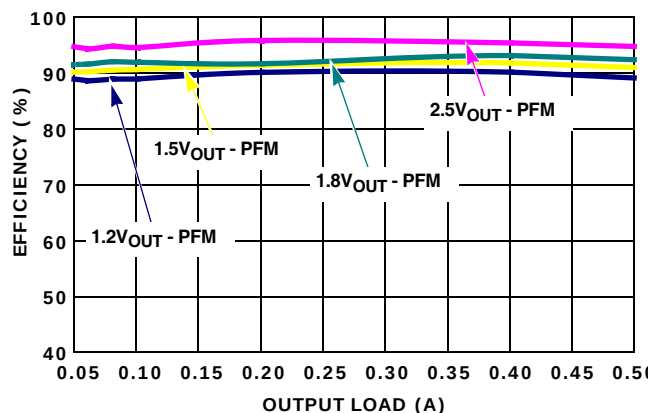
FIGURE 2. EFFICIENCY vs LOAD, V_{\text{IN}} = 3.3\text{V} PFM
