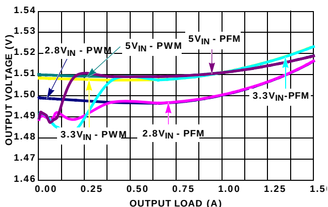
FIGURE 6. V_{\text{OUT}} REGULATION vs LOAD, V_{\text{OUT}} = 1.5\text{V}
