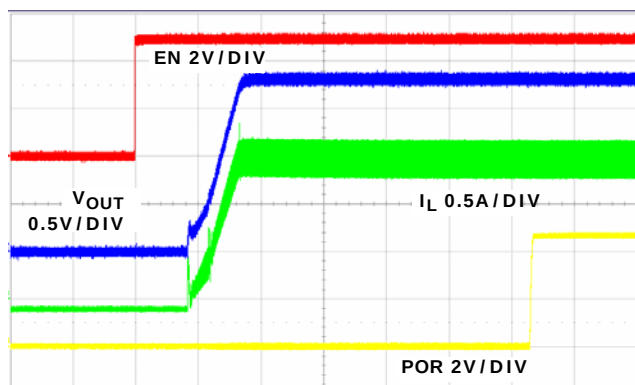
FIGURE 21. SOFT-START AT FULL LOAD, 500µs/DIV
