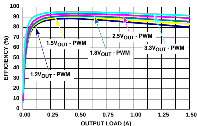
FIGURE 3. EFFICIENCY vs LOAD, V_{\text{IN}} = 5\text{V} PWM
