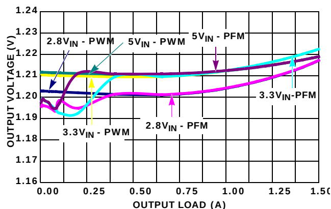
FIGURE 5. V_{\text{OUT}} REGULATION vs LOAD, V_{\text{OUT}} = 1.2\text{V}
