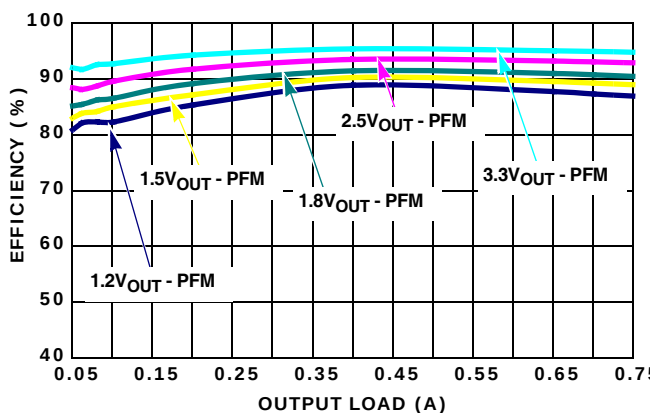
FIGURE 4. EFFICIENCY vs LOAD, V_{\text{IN}} = 5\text{V} PFM
