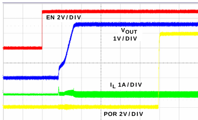
FIGURE 19. SOFT-START AT NO LOAD, 500µs/DIV
