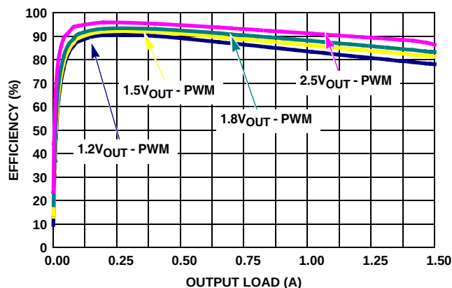
FIGURE 1. EFFICIENCY vs LOAD, V_{\text{IN}} = 3.3\text{V} PWM
