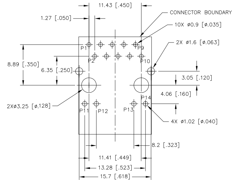
RECOMMENDED PWB LAYOUT (COMPONENT SIDE SHOWN)
