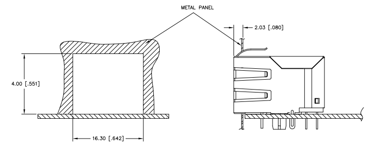
SUGGESTED PANEL CUTOUT
